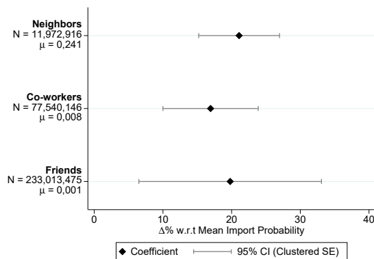
Figure 3: 2SLS: Propagation Within Network
