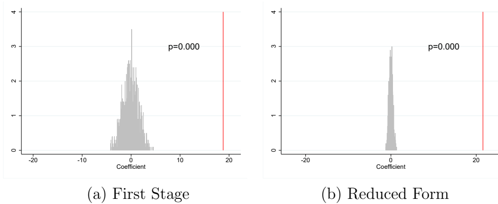
Figure 5: Placebo vs. Actual Coefficients
