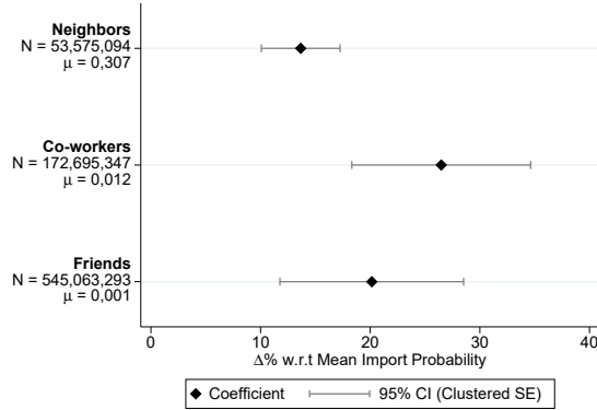
Figure D.3: 2SLS: Propagation Within Network (Instrument based on U.S. imports data)
